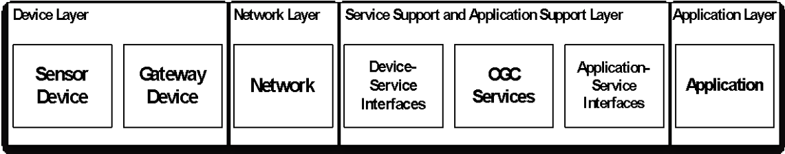
Figure 2 - IoT Reference Model and the Sub-layers
