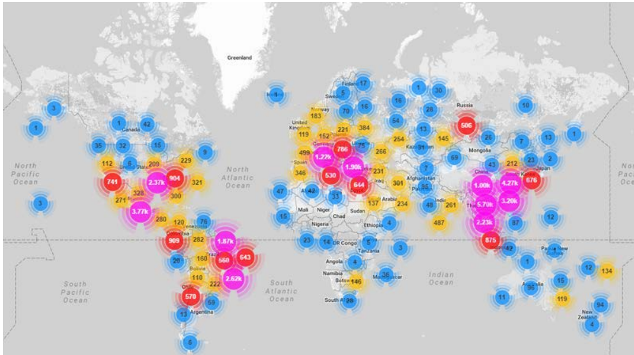
Figure 6. Traffic Sources for a Mirai Botnet Attack August 17, 2016
