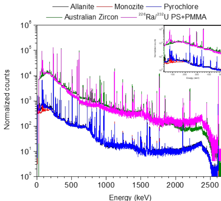
Figure 3 - Spectra of different NORM samples and simulated NORM using ^{226}\text{Ra} and ^{232}\text{U} point sources surrounded by 3.8 cm of PMMA
