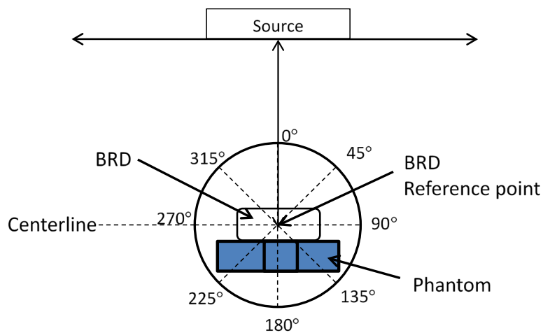
Figure 2 - Definition of testing angles when source passes at an angle of 0° (top view)
