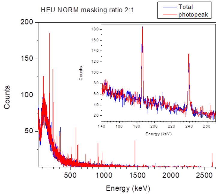
Figure 5 - HPGe spectra for HEU source masked with sand, masking ratio calculated using regions of interest and total flux, masking ratio 2:1.
