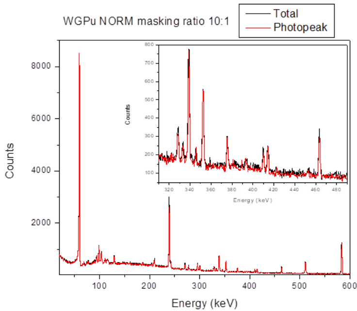
Figure 6 - HPGe Spectra for WGPu source masked with sand, masking ratio calculated using regions of interest and total flux, masking ratio 10:1
