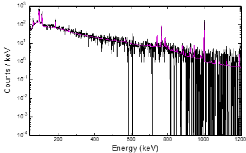
Figure 8 - Measured and GADRAS-generated DU plate spectrum
